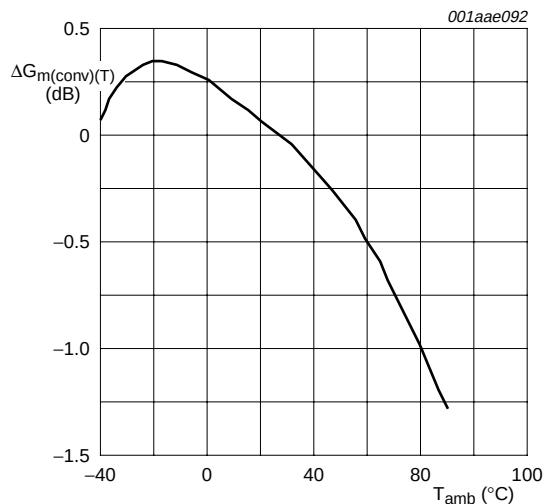
Fig 21. FM mixer conversion transconductance gain deviation over temperature (including application)
